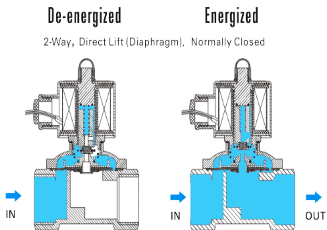
Fig 5: Section view of solenoid valve
