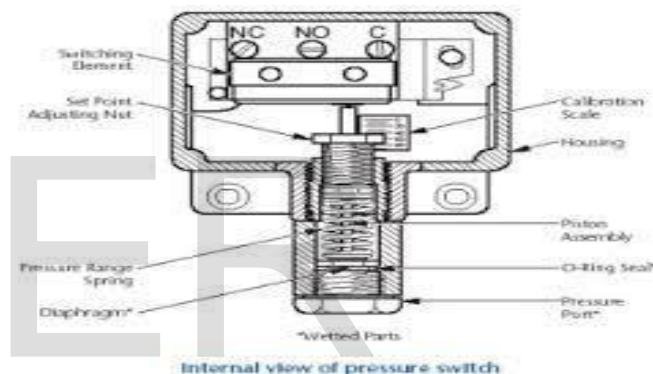
Fig 4: Internal view of pressure switch
